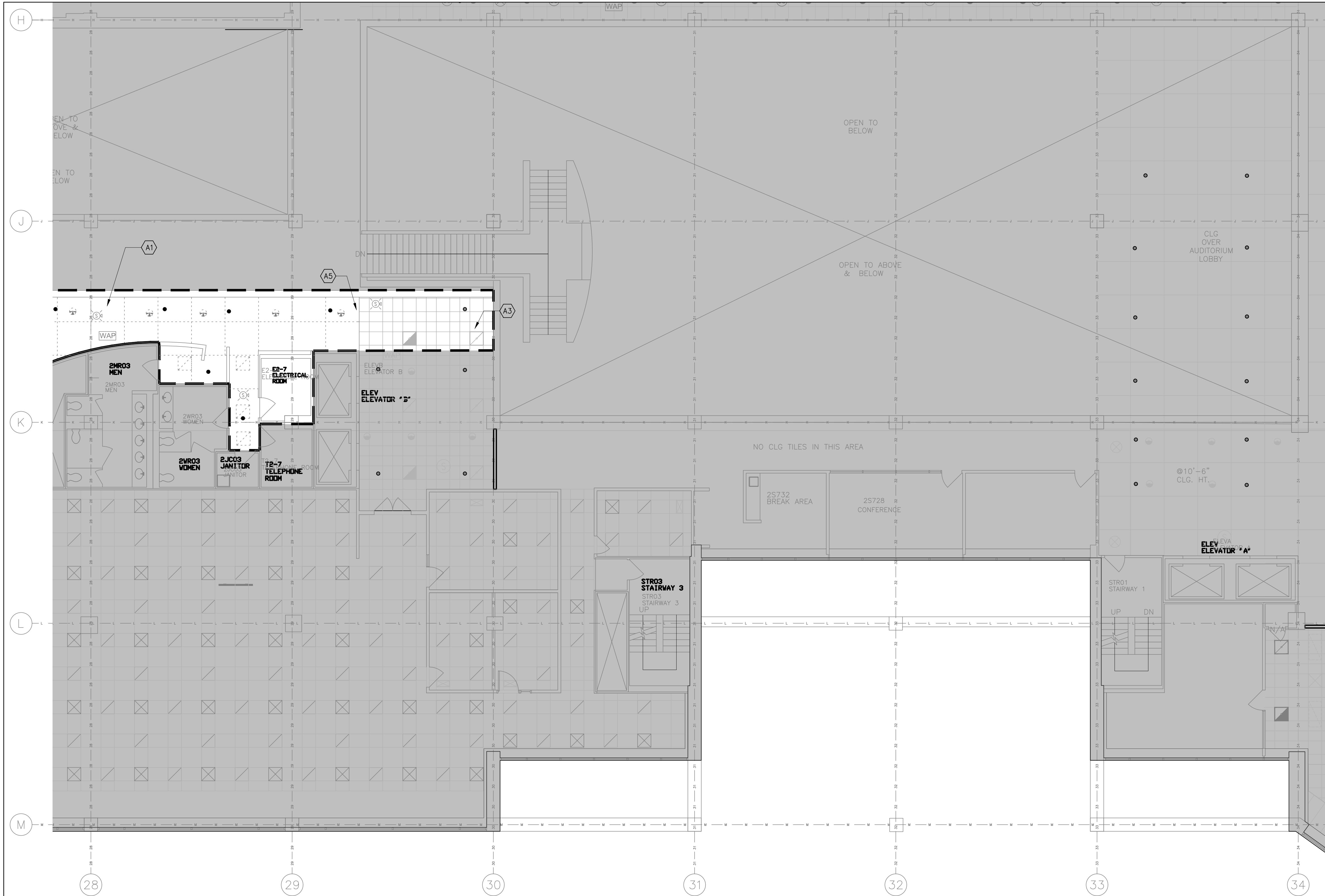
C PARTIAL SECOND FLOOR DEMOLITION REFLECTED CEILING PLAN - AREA "B" AD2.02 SCALE: 1/8" = 1'-0"
